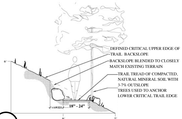
SECTION DETAIL: SINGLETRACK TYP.
