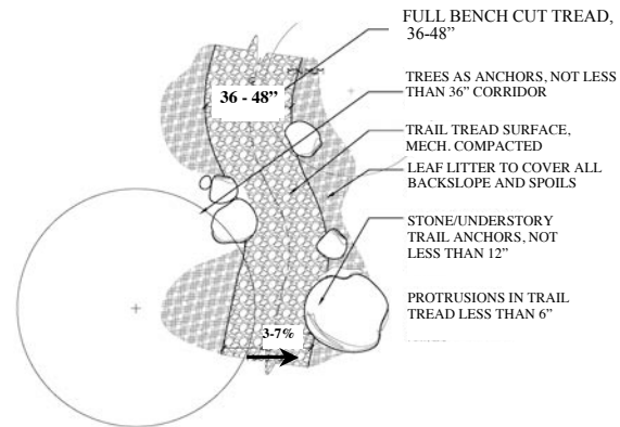
PLAN DETAIL: BACKCOUNTRY TRAIL TYP.
