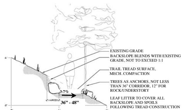
SECTION DETAIL: BACKCOUNTRY TRAIL- TYP.
