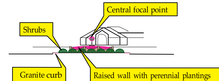
SECTION AT THE ATRIUM CIRCLE
