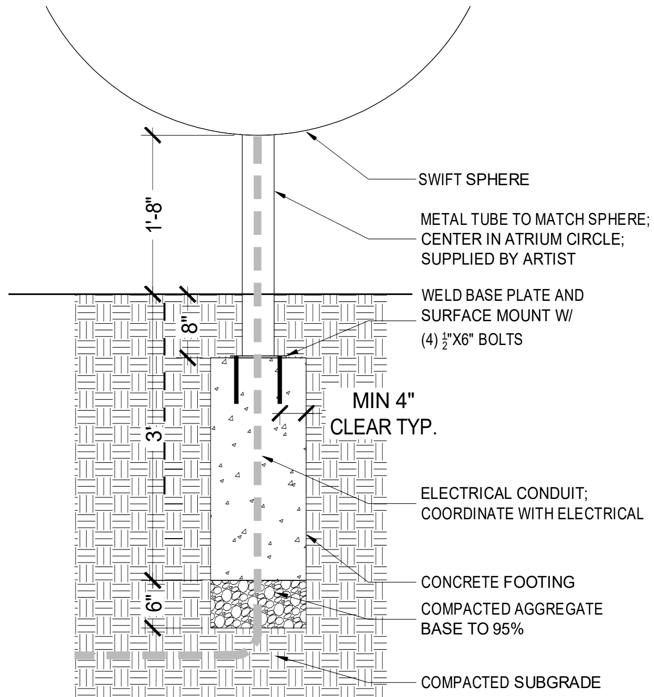
SWIFT SPHERE INSTALLATION 1"=1'
